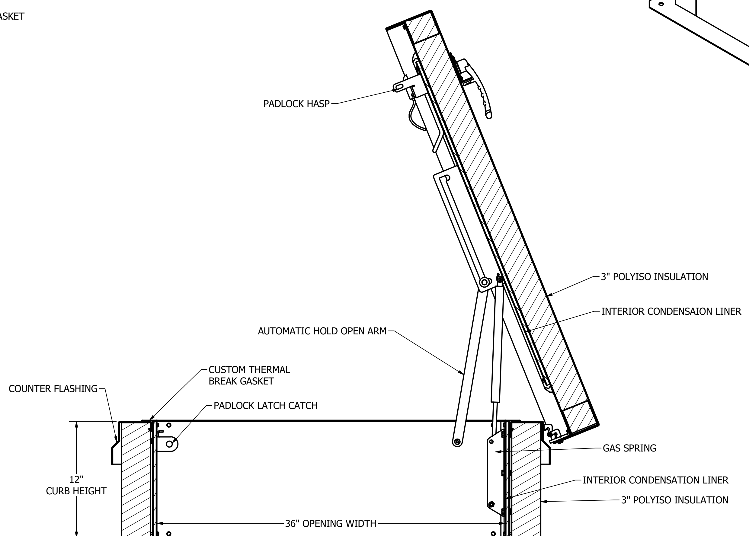
SECTION D-D SCALE 1/6
