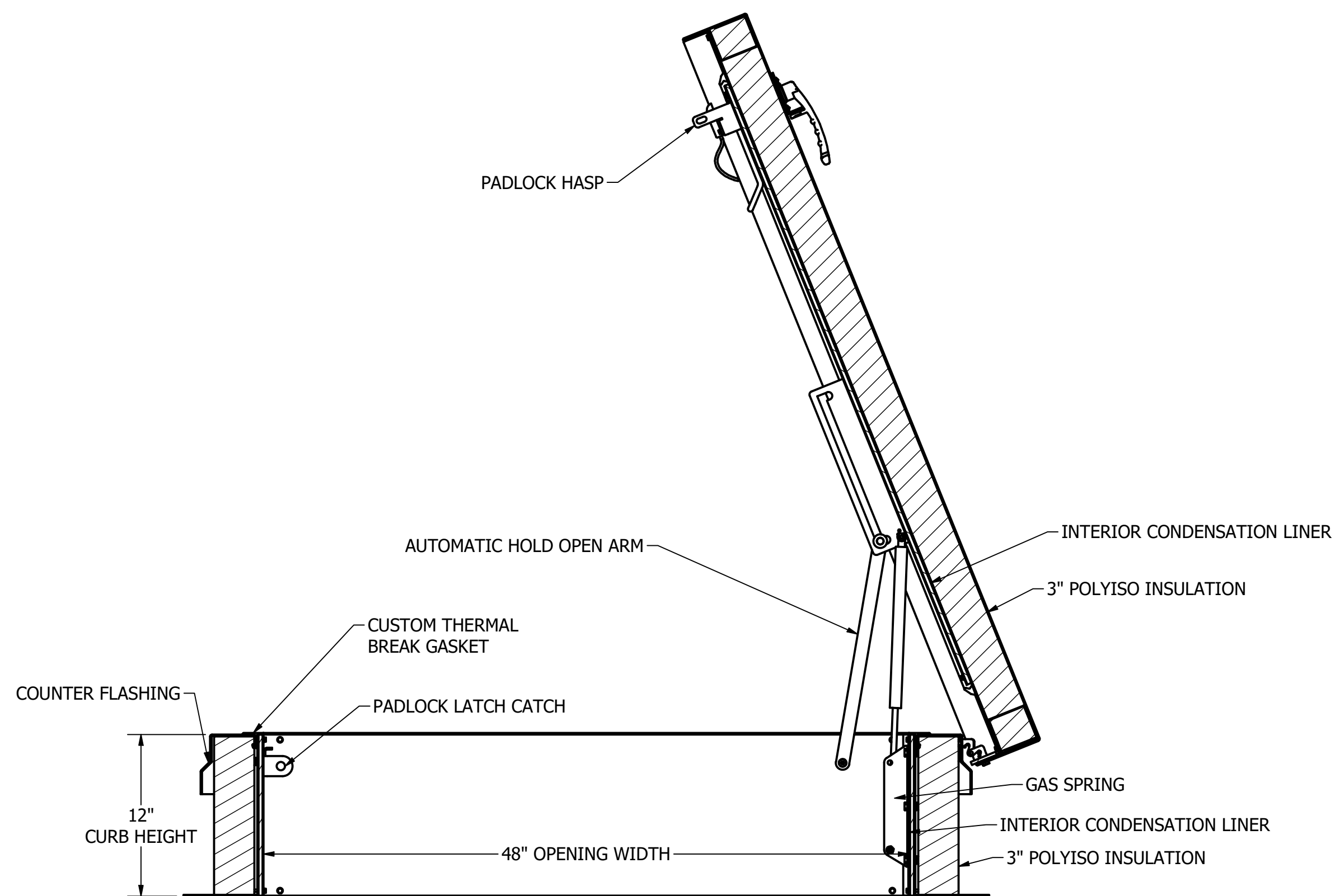
SECTION E-E SCALE 1/8
